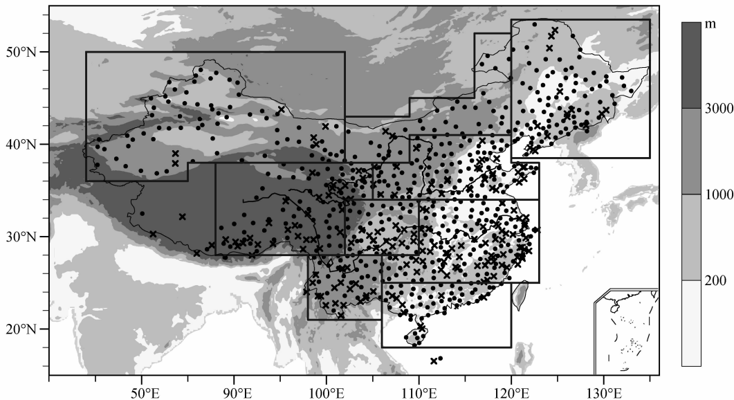
图 1 台站位置和区划分布示意图。黑点:本文选用的 559 站位置;叉点:剔除台站的位置;阴影:地形分布(单位:m) Fig. 1 Topographic distribution (shaded) over China, together with locations of rain gauge stations used (559 stations, closed circle) and rejected (cross mark) in this paper. Nine sub-regions are outlined for regional averaging
