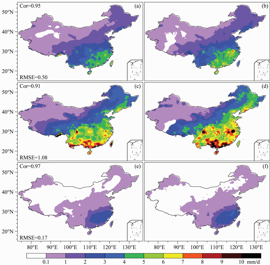
图2 (a、b)年平均和(c、d)夏季和(e、f)冬季平均降水的空间分布(单位: mm/d): (a、c、e) APHRO 资料(左上角数值表示两套降水资料的空间相关系数,左下角数值表示二者的均方根误差); (b、d、f) STN 资料 Fig.2 Spatial distributions of the average (a, b) annual, (c, d) summer, and (e, f) winter precipitation amount during 1956–2005 from (a, c, e) APHRO data and (b, d, f) STN data. The numbers shown in the upper corners in (a, c, e) indicate pattern correlation coefficients with STN data; the numbers shown in the lower corners in (a, c, e) indicate root mean square error with STN data
