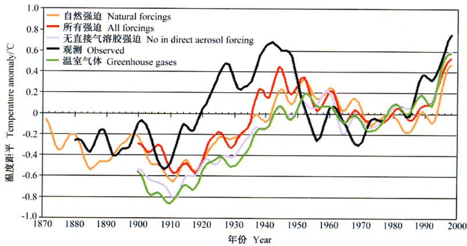
图 4 用英国模式 HADL 考虑太阳活动、火山活动和人类活动模拟的近百余年中中国年平均气温距平变化 (其中黑线是观测值) [1, 24] Fig. 4 Annual mean temperature anomalies in China for the 20th century as simulated by the HADL AOGCM with solar, volcanic and human activities (black curve is observation) [1, 24]
