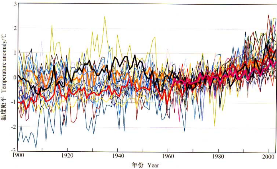
图 6 大约 40 个气候模式和试验设计模拟的 20 世纪中国年平均表面气温距平的变化以及相应的观测变化（相对于 1961~1990 年。粗红线为 GCM7 GG，粗黄线为 GCM7 GS，粗深紫色线为 GCM7 SRES A2，粗浅紫色实线是 GCM7-SRES B2，粗黑实线是观测值。在文献 [4, 6, 25~27] 基础上发展） Fig. 6 Annual mean temperature anomalies in China for the 20th century as simulated by the climate models with several scenarios (relative to 1961—1990, thick red curve is GCM7-GG, thick-dark yellow curve is GCM7-GS, thick-dark purple curve is SRES A2, thick-light purple curve is SRESB2, thick-black curve is observation, based on [4, 6, 25~27]) (气候模式和试验设计 Climate models with several scenarios; CCC-GG, CCSR/NIES GG, CSIRO-GG, DKRZ-GG, GFDL-GG, HADL-GG, NCAR-GG, GCM7-GG, CCC-GS, CCSR/NIES-GS, CSIRO-GS, DKRZ-GS, GFDL-GS, HADL-GS, NCAR-GS, GCM7-GS, LASG/IAP-GG, LASG-IAP-GS, LASG-IAP-GSS, NCC/IAP T63-GG, NCC/IAP T63 GS, CCSR/NIES2 A1, A2, B1, B2, CCC-A2, CSIRO-A2, ECHAM A2, GFDL-A2, HADL A2, CCC-B2, CSIRO-B2, ECHAM-B2, GFDL B2, HADL-B2, GCM14 SRES, NCC/IAP T63-A2, NCC/IAP T63-B2)
