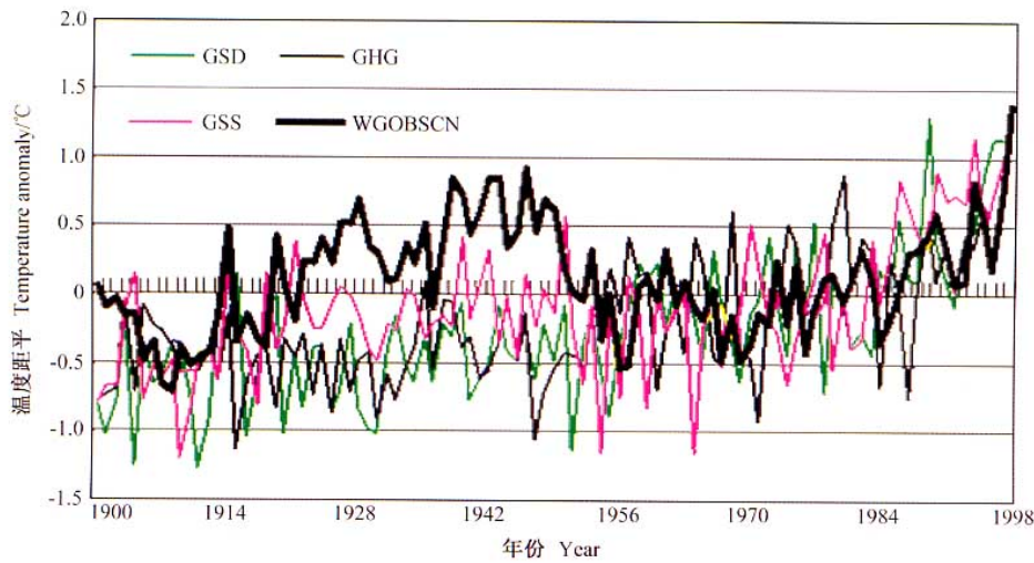
图 3 中国科学院大气物理研究所模式 (GOALS/LASG) 考虑温室气体 (GHG)、温室气体+硫酸盐气溶胶 (GS)、温室气体+硫酸盐气溶胶+太阳活动 (GSS), 模拟 20 世纪中国年平均气温变化 (粗黑线是观测值 WGOBSCN) [4] Fig. 3 Annual mean temperature anomalies in China for the 20th century as simulated by the GOALS/LASG AGCM with scenarios of GHG, GS, GSS (black curve is observation) [4]
