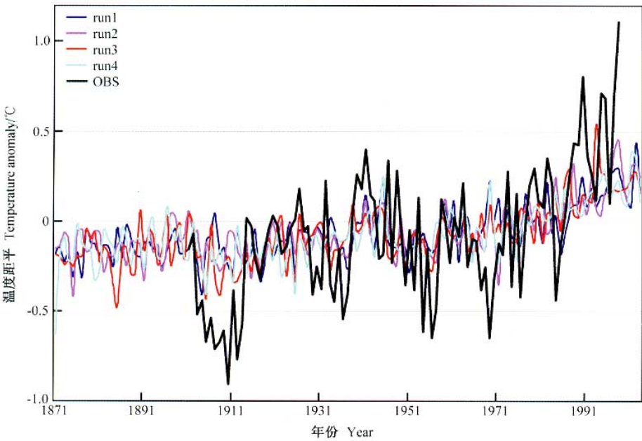
图 5 中国气象局国家气候中心全球大气环流模式（NCC T63）考虑太阳活动、温室气体和平流层臭氧，在观测海温和海冰驱动下，模拟 20 世纪东亚地区气温距平变化（其中黑线是观测值） [7] Fig. 5 Annual mean temperature anomalies over East Asia for the 20th century as simulated by the NCC T63 AGCM with radiative forcing and observed SST and sea ice (black curve is observation) [7]
