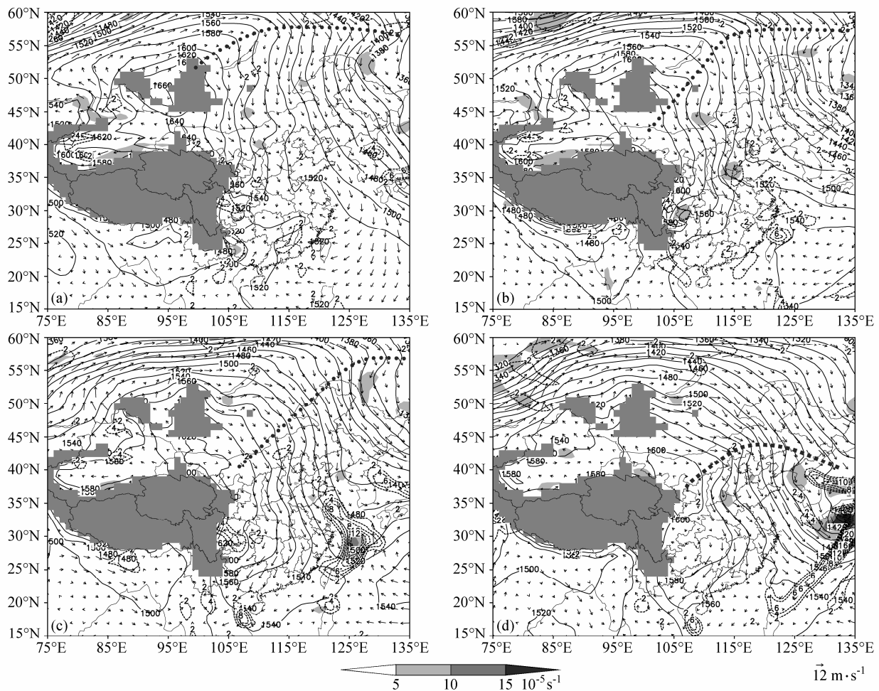
图 4 850 hPa 形势图,包括 850 hPa 涡度(阴影)、位势高度(实线,单位: gpm)、水平风场(箭头)和垂直速度(虚线,单位: 10^{-2} m/s): (a) 2004 年 12 月 29 日 12:00; (b) 30 日 00:00; (c) 30 日 12:00; (d) 31 日 00:00。地形高度超过 1500 m 用小正方形填充,粗点线为脊线 Fig. 4 Vorticity (shaded), geopotential (solid line, units: gpm), horizontal wind (vector), and vertical velocity (dashed line, units: 10^{-2} m/s) at 850 hPa, terrain above 1500 m is filled with grey square and thick dashed line indicates ridge line: (a) 1200 UTC 29 Dec 2004; (b) 0000 UTC 30 Dec 2004; (c) 1200 UTC 30 Dec 2004; (d) 0000 UTC 31 Dec 2004
