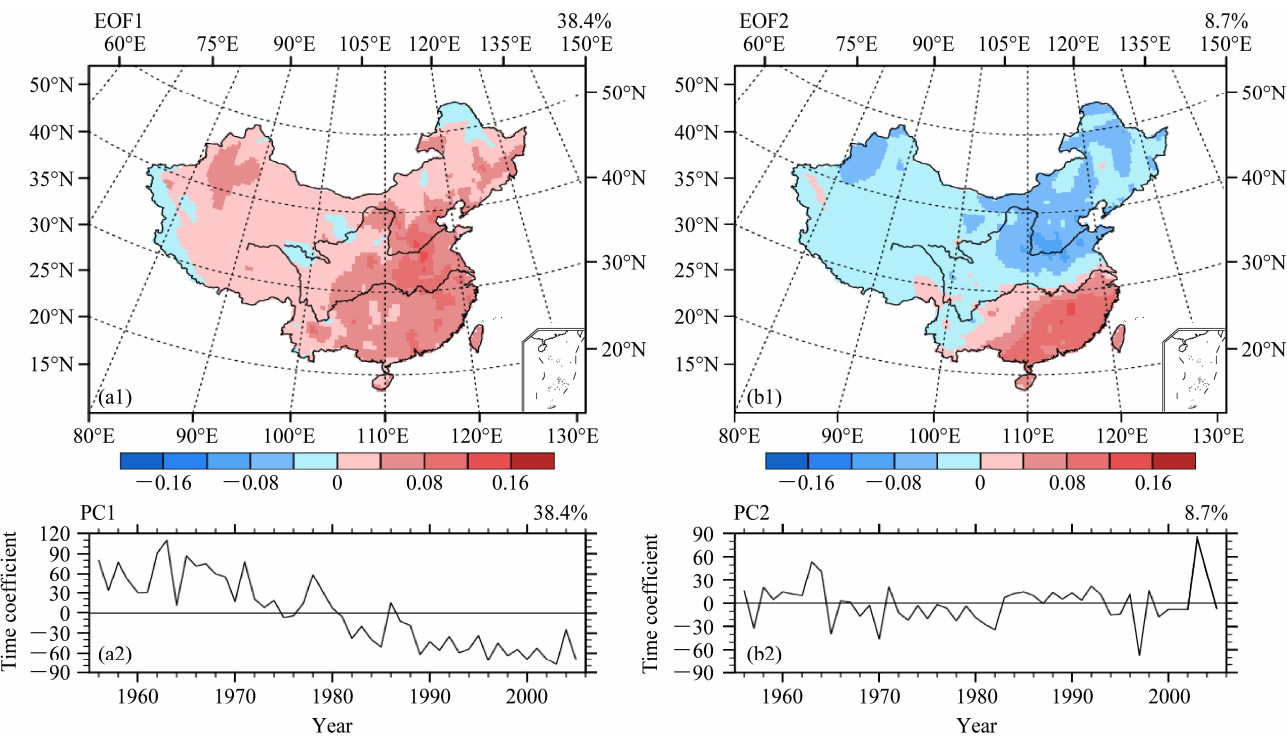
图 5 EOF 分解后的第一分量图（左列）与第二分量图（右列）对应的（a1、b1）空间模态和（a2、b2）时间系数 Fig. 5 The (a1, b1) leading EOF eigenvectors and (a2, b2) temporal coefficient of sunshine duration at 309 stations in China for EOF1 (left column) and EOF2 (right column)
